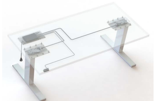
Fig. 6: Application example: mounting of telescopic legs for a stand-up table system
