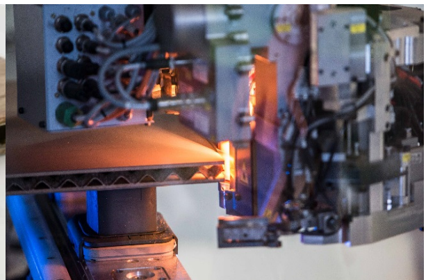
Free-form machining and edging without supporting edge
