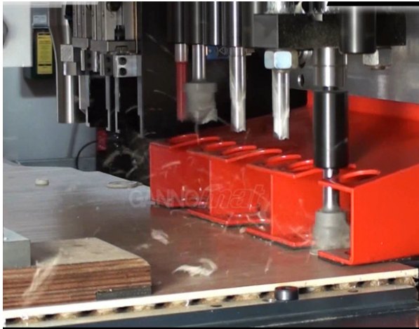
Drilling and milling on a machining centre
