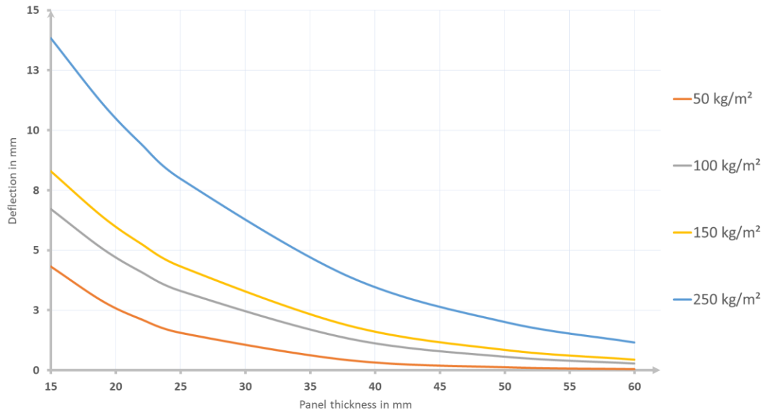
Average deflection as a function of panel thickness and applied test load; span 800 mm
